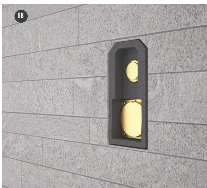
After removing the built-in box front cover, remove the cover exceeding the edge of the wall with a cutter.
